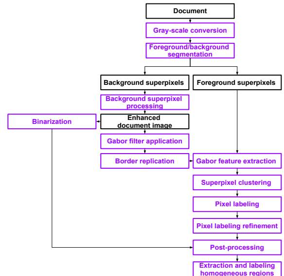
Figure 1: Flowchart of the proposed algorithm for extraction of homogeneous regions in HDIs.
