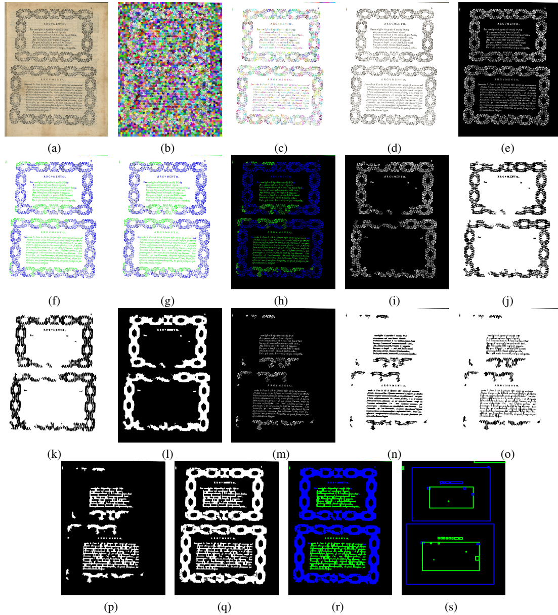
Figure 3: Illustration of the intermediate results of the different tasks of the proposed algorithm: Figure (a) shows an example of an HDI (as an input of the proposed algorithm). Figures (b) and (c) show the background and foreground SLIC superpixels, respectively. Colors assigned to the background (foreground, respectively) superpixels which are illustrated in Figure (b) ((c), respectively) are randomly generated. Figure (d) depicts the result of the enhancement step. Figure (e) shows the resulting image of applying a binarization step on the enhanced document image. Figure (f) illustrates the pixel-labeled image (as an output of the analysis of the extracted Gabor features (graphic regions (blue), textual regions (green))). Figure (g) depicts the results of the pixel labeling refinement step. Figure (h) shows the resulting image of the labeling of the extracted CCs from the binarized enhanced document image according to the obtained pixel labeling results in the pixel labeling refinement step by using the majority voting technique. Figures (i) and (m) are the two resulting binarized images of the color layer separation task, illustrating separately the graphical (blue) and textual (green) CCs, respectively. Figures (j) and (k) show the resulting images of the application of the run-length smearing both horizontally and vertically on the resulting binarized image representing the graphical regions ( cf. Figure (i)), respectively. Figures (n) and (o) show the resulting images of the application of the run-length smearing both horizontally and vertically on the resulting binarized image representing the textual regions ( cf. Figure (m)), respectively. Figure (l) ((p), respectively) is the resulting image of merging the two resulting images of applying the run-length smearing both horizontally and vertically on each resulting binarized image of the color layer separation task ( cf. Figures (j) and (k)) ( cf. Figures (n) and (o), respectively) by using the logical OR . Figure (q) is the resulting image of merging the two resulting images of applying ARLSA on each resulting binarized image of the color layer separation task by using the logical OR ( cf. Figures (l) and (p), respectively). Figure (r) shows the resulting image of the post-processing step by labeling the extracted CCs from Figure (q) with taking into account the labels of the extracted CCs from Figure (h). Figure (s) illustrates the output of the proposed algorithm for extraction of homogeneous regions in HDIs.
