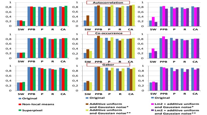
Fig. 3. Evaluation of the extracted textural features using different accuracy metrics on enhanced images (non-local means filtering and superpixel techniques) and degraded images: silhouette width (SW), purity per block (PPB), precision (P), recall (R), and classification accuracy (CA). The "*" and "**" represent the case when the clustering is performed by setting the number of types of content regions equal to the defined one on the ground-truth, and to the defined one on the ground-truth +1 ( i.e. the noisy foreground cluster has been taken into account) respectively.
