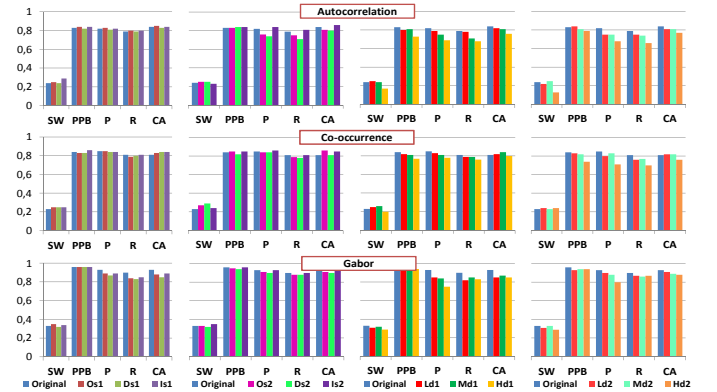
Fig. 4. Evaluation of the extracted features on degraded images under different degradation models: silhouette width (SW), purity per block (PPB), precision (P), recall (R), and classification accuracy (CA).
