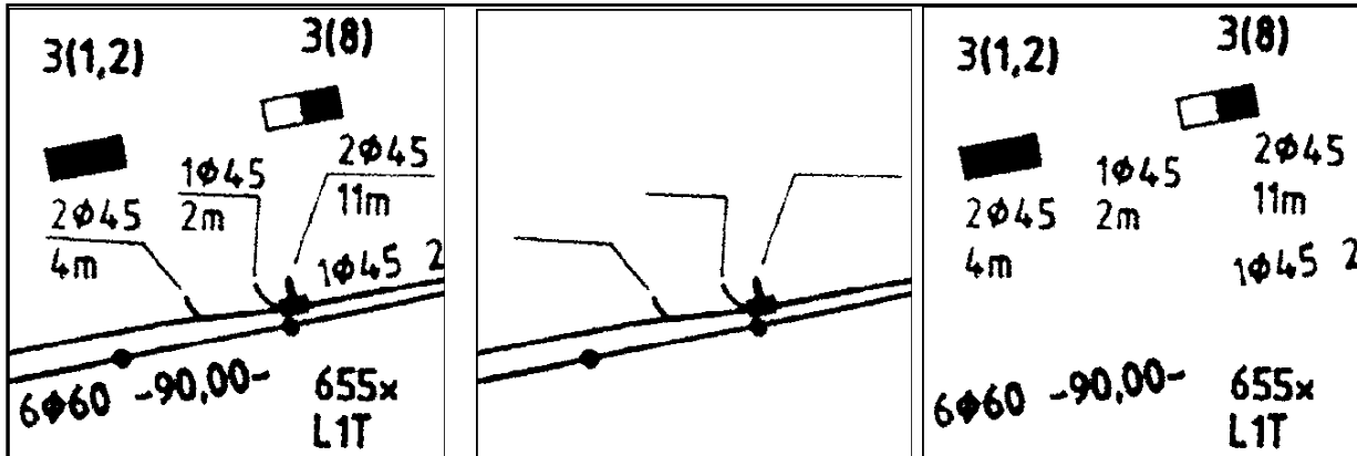
Figure 9.1 : Original image
