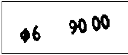
Figure 13.1 : Connected characters
