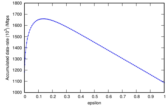
Fig. 5. Exploitation-exploration trade-off.
