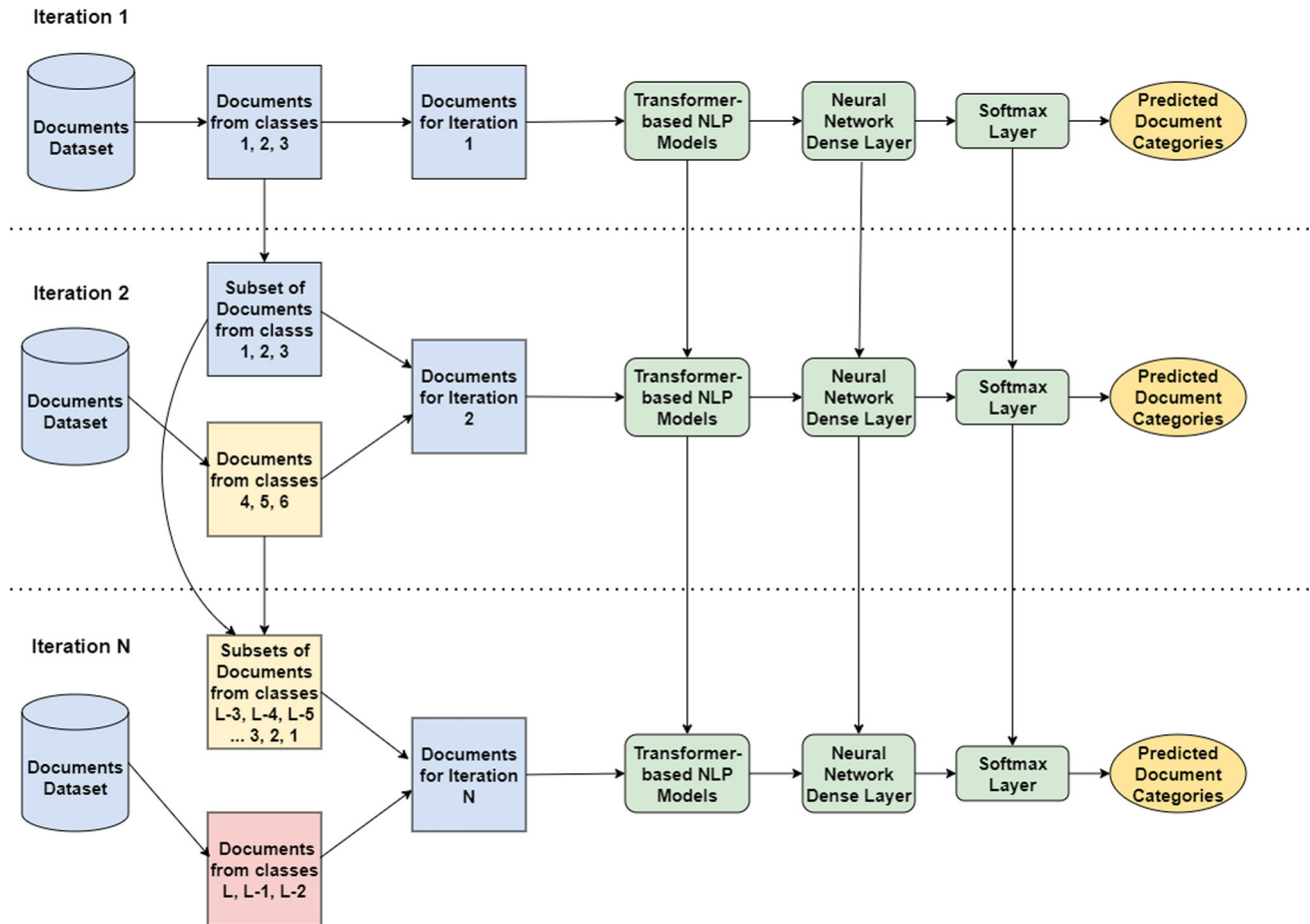
Fig. 2 Proposed approach for rehearsal-based incremental document classification. In this diagram, the number of initial classes (BC) and new classes per iteration (NC) is arbitrarily set to 3. L represents the total number of classes. N represents the total number of training iterations
